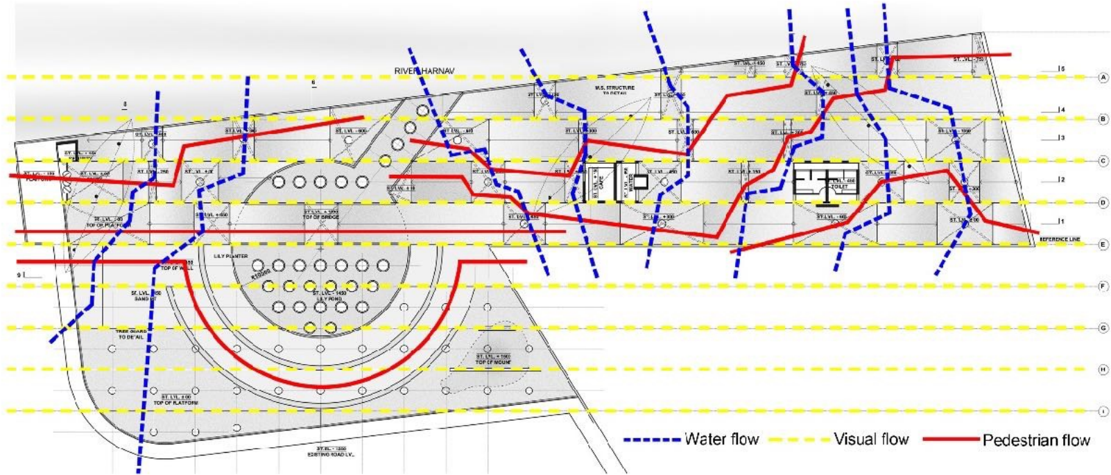
Each Slope is meticulously designed to channelise the water movement from one walkway to other & then into the river
